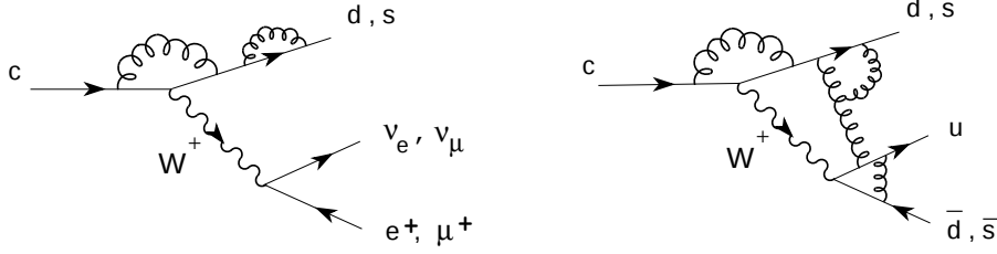
Fig. 31: Determinations of V_{ij} are done in semileptonic quark decays (left), where a single quark current is present. Hadronic decay modes (right) involve two different quark currents and are more affected by QCD effects (gluons can couple everywhere).
