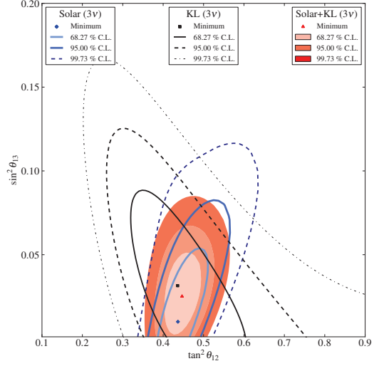
Fig. 35: Allowed regions for three-flavour neutrino oscillations, using both solar neutrino and KamLAND (KL) results, assuming \mathcal{CPT} symmetry [105].
