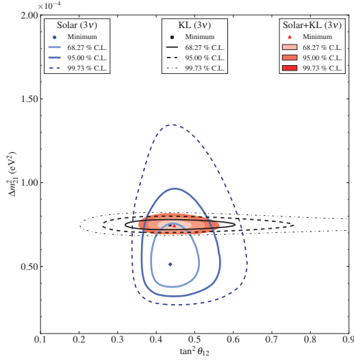
Fig. 35: Allowed regions for three-flavour neutrino oscillations, using both solar neutrino and KamLAND (KL) results, assuming \mathcal{CPT} symmetry [105].
