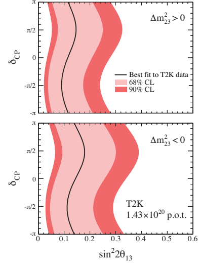
Fig. 37: Constraints on \sin^2(2\theta_{13}) versus the \mathcal{CP} phase \delta_{CP} \equiv \delta_{13} from T2K data [116].
