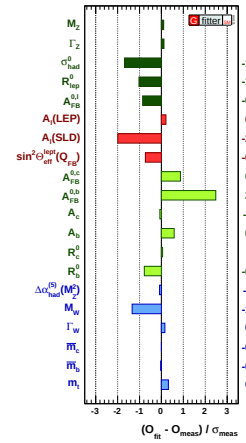
Fig. 25: Comparison between the measurements included in the combined analysis of the SM and the results from the global electroweak fit [55].
