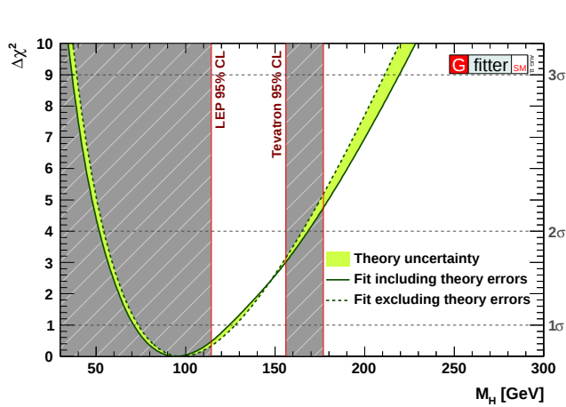
Fig. 24: \Delta\chi^2 versus M_H , from the global fit to the electroweak data. The vertical bands indicate the 95% exclusion limits from direct searches [55].
