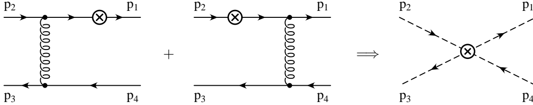
FIG. 2: Tree level matching onto C_{0,8} . The QCD graphs on the left plus the analogous graphs with the current on the bottom quark line are matched onto the collinear operator on the right.
