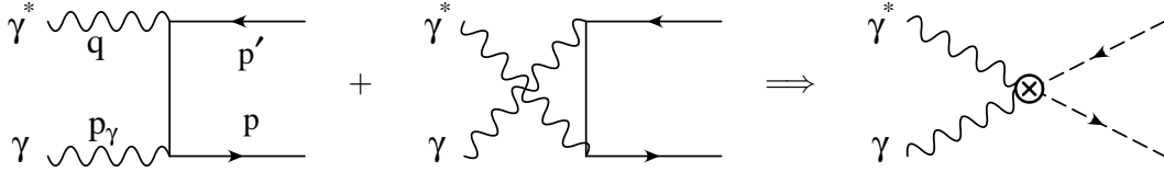
FIG. 1: Tree level matching onto O_j in the Breit Frame. The graphs on the left include u and d quarks.
