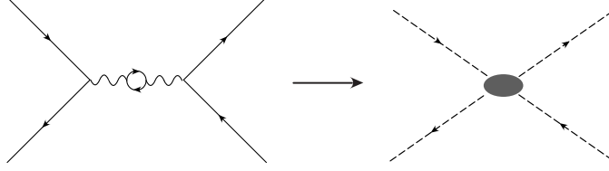
FIG. 4: Tree level matching onto the operators in Drell-Yan.
