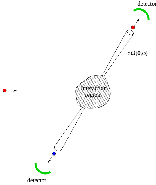
Fig. 10: Schematic setup of a two-to-two-particles single scattering event in the center of mass reference frame.
