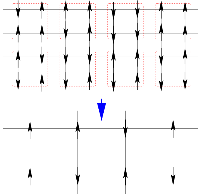
Fig. 16: Decimation of the spin lattice. Each block in the upper lattice is replaced by an effective spin computed according to the rule (8.32). Notice also that the size of the lattice spacing is doubled in the process.
